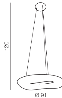
Donut Pendant CCT 91 LED
