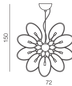
Diana 16 AZ2155 G9 16x MAX 40W glass/metal
